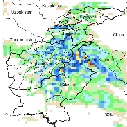
Daily Precip. Forecast for 22 Feb., 2013
