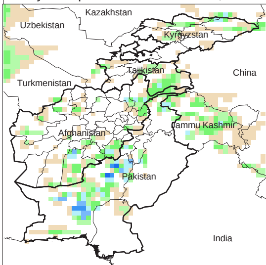
Daily Precip. Forecast for 20 Feb., 2013
