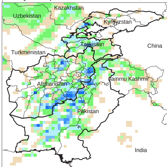
Daily Precip. Forecast for 21 Feb., 2013
