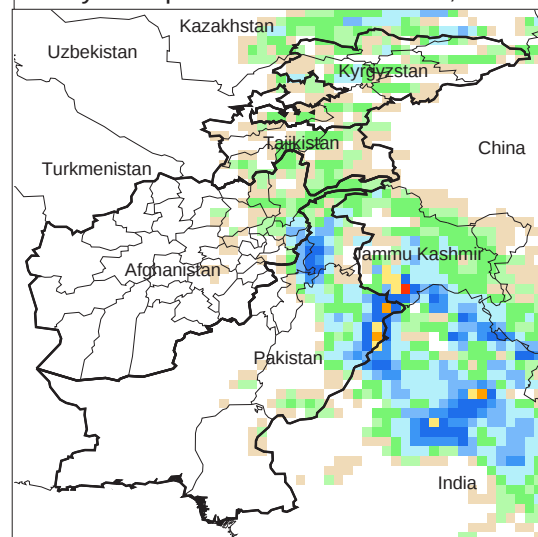
Daily Precip. Forecast for 23 Feb., 2013
