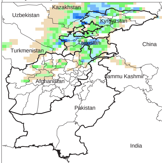
Daily Precip. Forecast for 3 Mar., 2013
