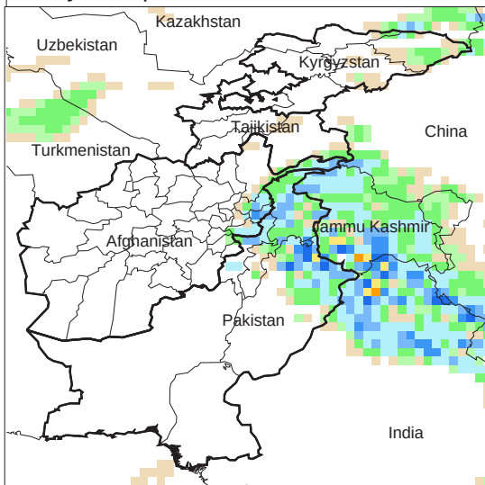
Daily Precip. Forecast for 17 Mar., 2013
