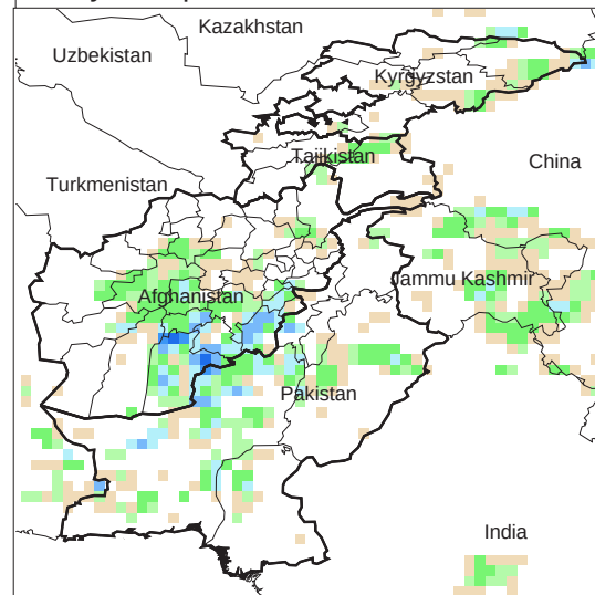
Daily Precip. Forecast for 27 Mar., 2013
