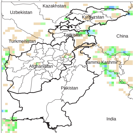
Daily Precip. Forecast for 25 Mar., 2013
