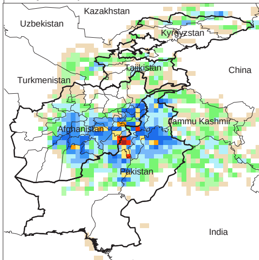
Daily Precip. Forecast for 26 Mar., 2013
