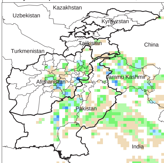
Daily Precip. Forecast for 28 Mar., 2013
