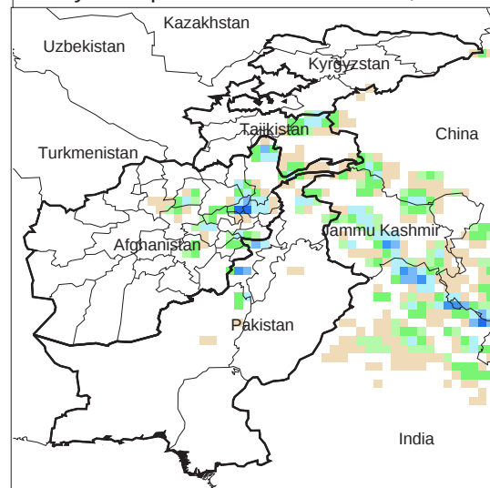
Daily Precip. Forecast for 29 Mar., 2013
