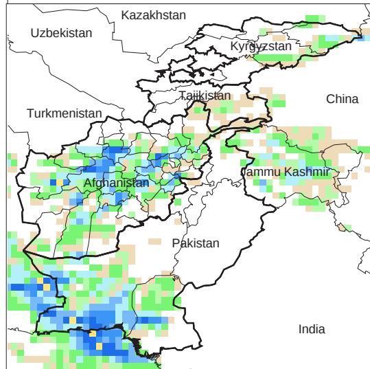
Daily Precip. Forecast for 11 Apr., 2013
