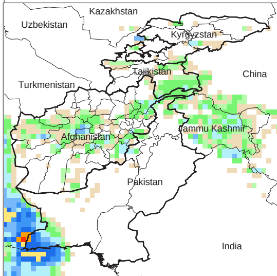
Daily Precip. Forecast for 10 Apr., 2013
