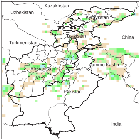
Daily Precip. Forecast for 9 Apr., 2013
