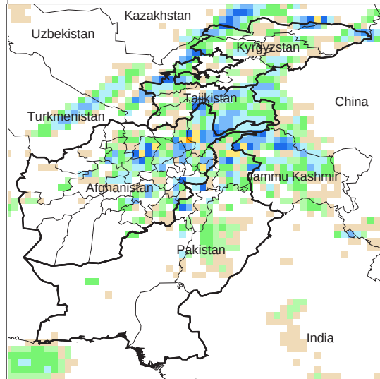
Daily Precip. Forecast for 29 Apr., 2013
