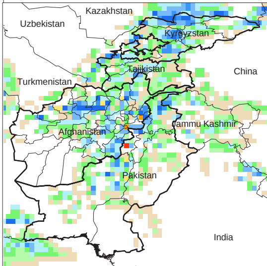
Daily Precip. Forecast for 27 Apr., 2013
