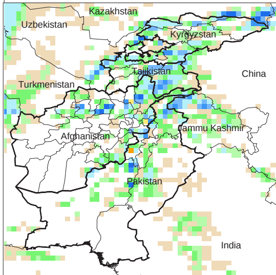
Daily Precip. Forecast for 28 Apr., 2013
