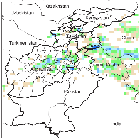
Daily Precip. Forecast for 9 May, 2013
