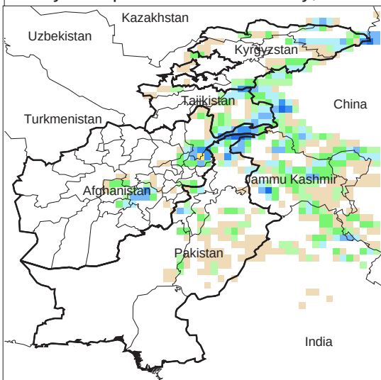
Daily Precip. Forecast for 10 May, 2013
