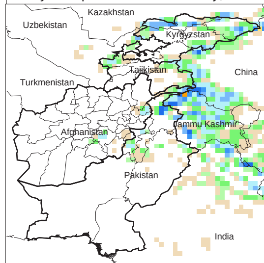
Daily Precip. Forecast for 11 May, 2013
