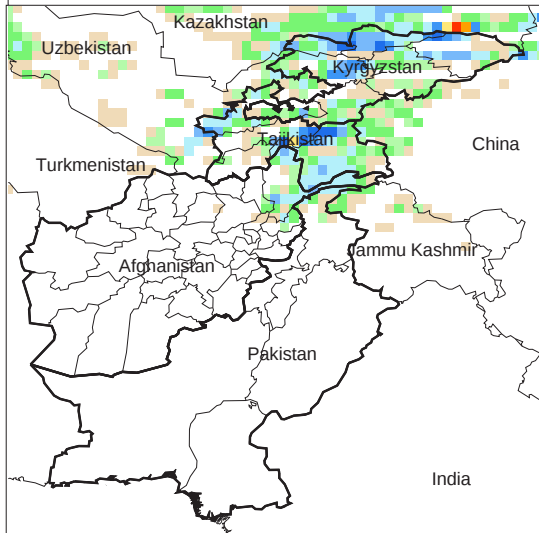
Daily Precip. Forecast for 19 May, 2013
