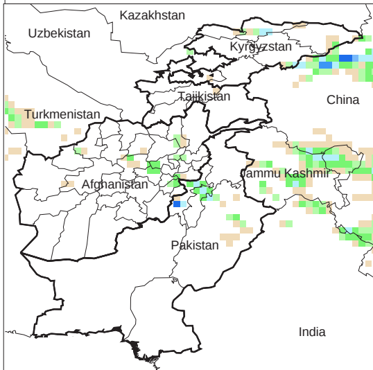
Daily Precip. Forecast for 18 May, 2013
