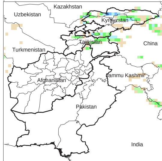
Daily Precip. Forecast for 20 May, 2013
