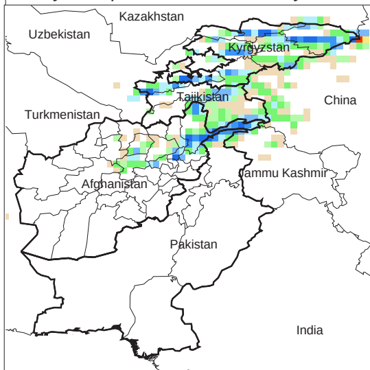
Daily Precip. Forecast for 24 May, 2013
