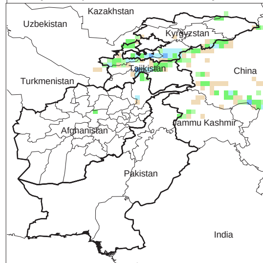
Daily Precip. Forecast for 25 May, 2013
