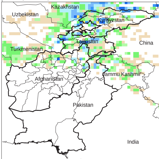
Daily Precip. Forecast for 23 May, 2013
