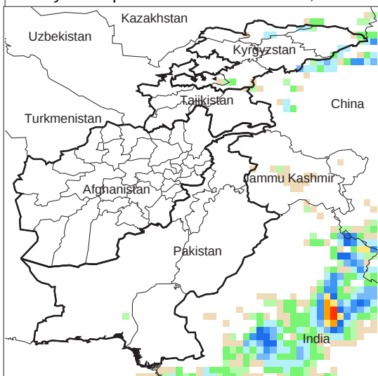
Daily Precip. Forecast for 19 Jun., 2013
