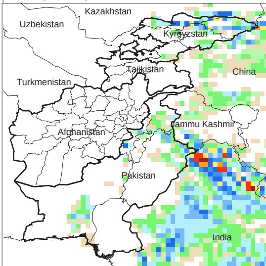
Daily Precip. Forecast for 10 Jul., 2013
