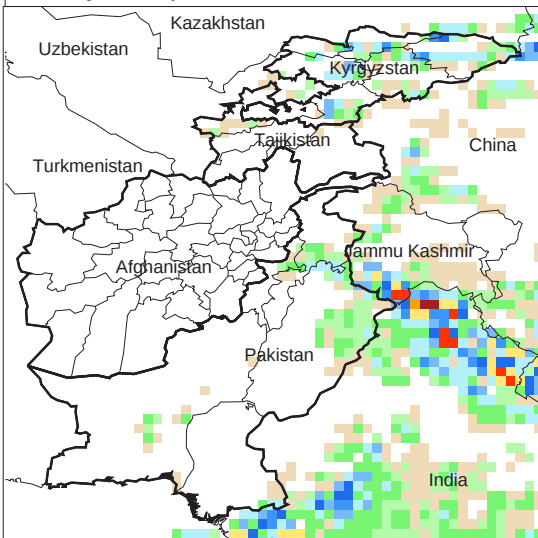
Daily Precip. Forecast for 9 Jul., 2013
