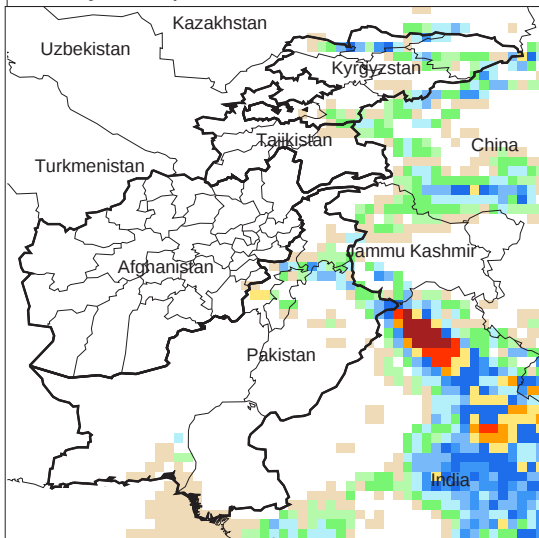
Daily Precip. Forecast for 11 Jul., 2013
