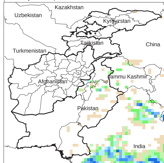
Daily Precip. Forecast for 4 Oct., 2013
