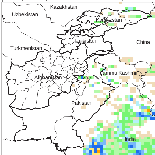
Daily Precip. Forecast for 3 Oct., 2013
