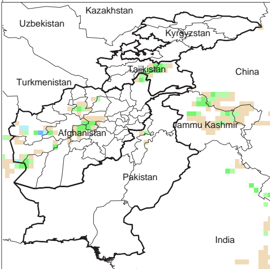
Daily Precip. Forecast for 18 Oct., 2013
