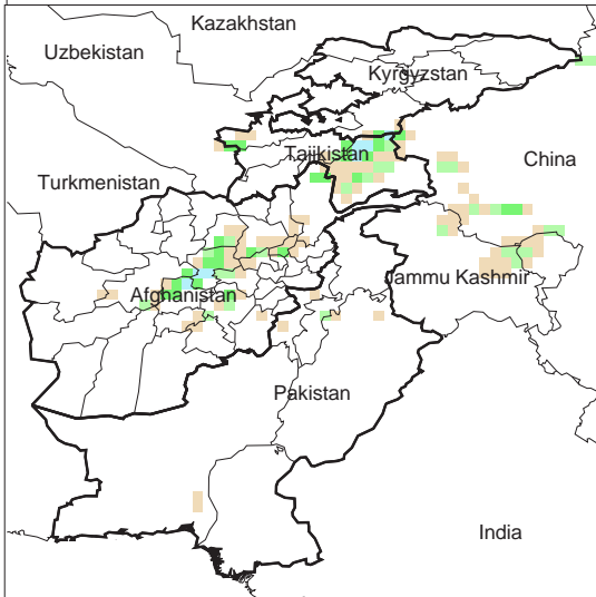
Daily Precip. Forecast for 19 Oct., 2013
