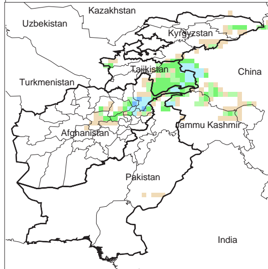
Daily Precip. Forecast for 20 Oct., 2013
