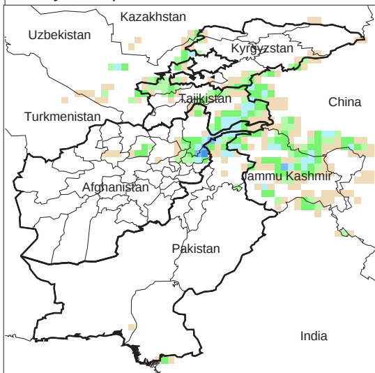
Daily Precip. Forecast for 31 Oct., 2013
