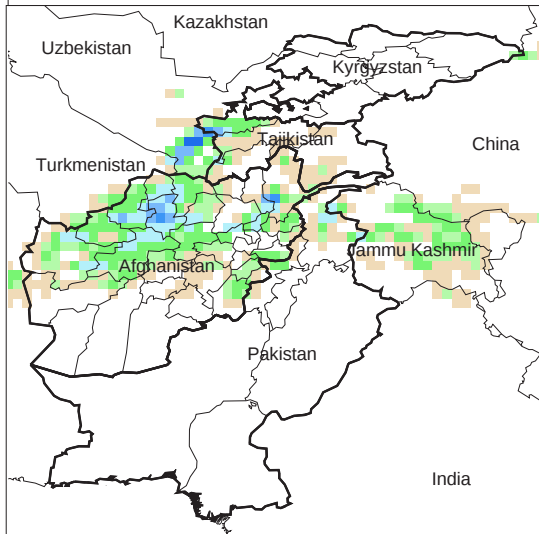
Daily Precip. Forecast for 1 Nov., 2013
