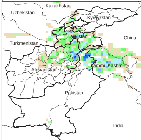
Daily Precip. Forecast for 2 Nov., 2013
