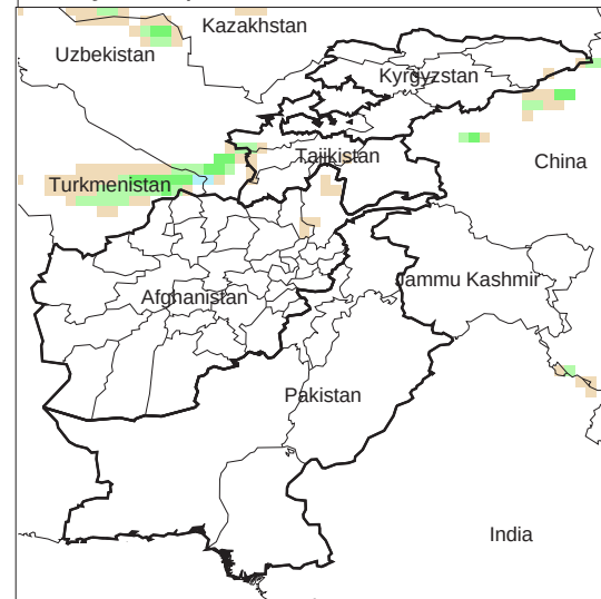
Daily Precip. Forecast for 13 Nov., 2013
