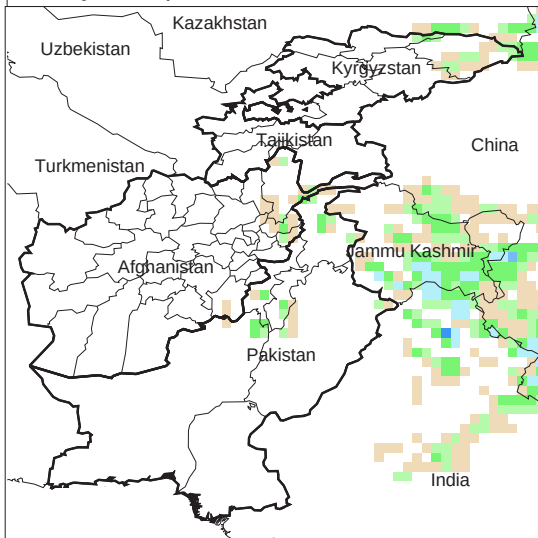
Daily Precip. Forecast for 11 Nov., 2013
