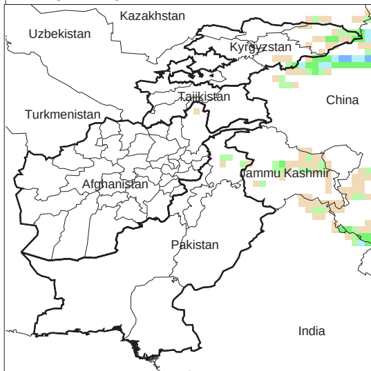
Daily Precip. Forecast for 12 Nov., 2013
