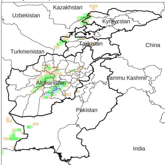
Daily Precip. Forecast for 16 Nov., 2013
