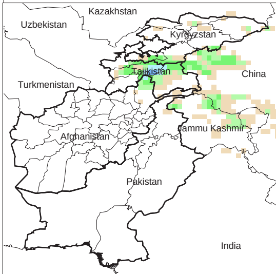
Daily Precip. Forecast for 15 Nov., 2013
