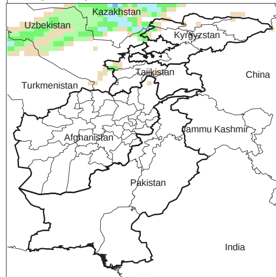
Daily Precip. Forecast for 2 Dec., 2013
