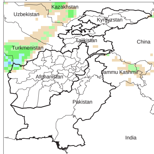
Daily Precip. Forecast for 3 Dec., 2013
