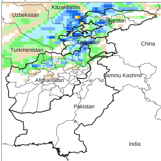
Daily Precip. Forecast for 1 Dec., 2013
