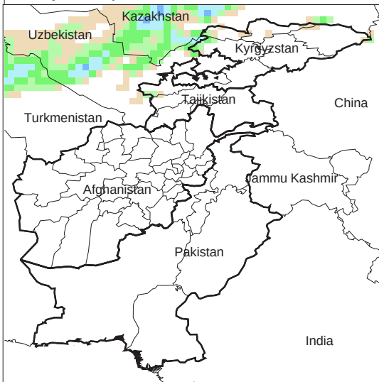
Daily Precip. Forecast for 2 Dec., 2013
