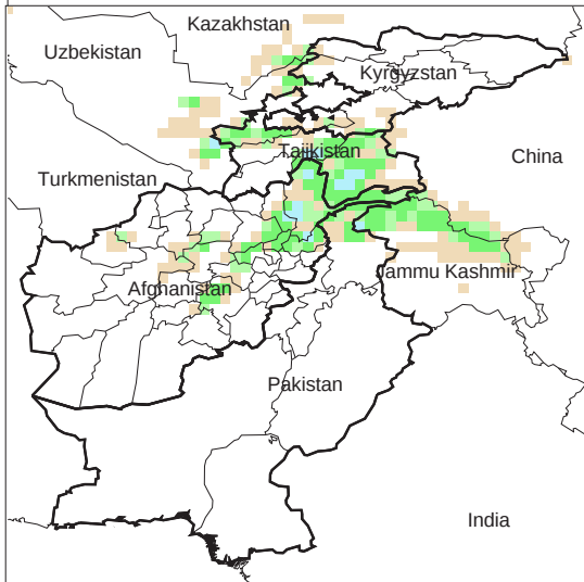
Daily Precip. Forecast for 3 Jan., 2014
