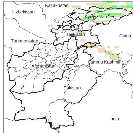
Daily Precip. Forecast for 5 Jan., 2014
