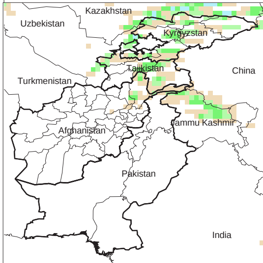
Daily Precip. Forecast for 4 Jan., 2014
