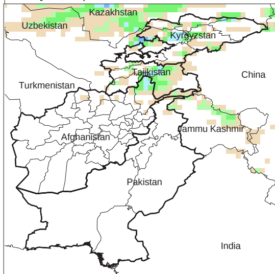
Daily Precip. Forecast for 29 Jan., 2014
