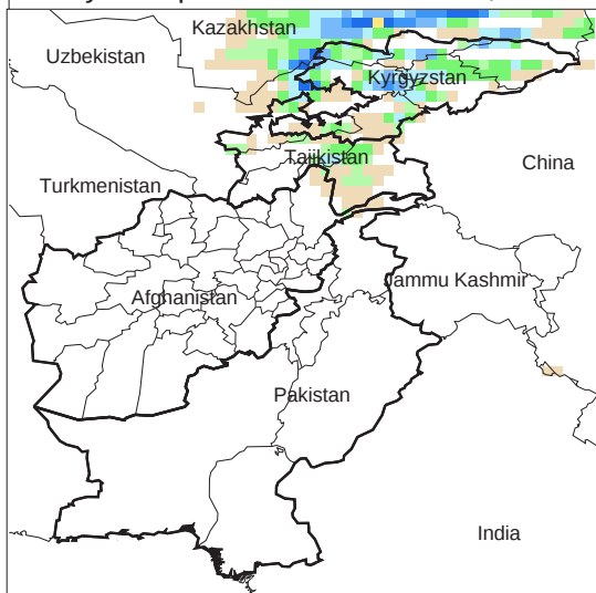
Daily Precip. Forecast for 28 Jan., 2014
