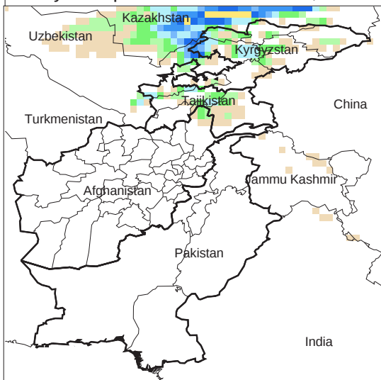
Daily Precip. Forecast for 27 Jan., 2014
