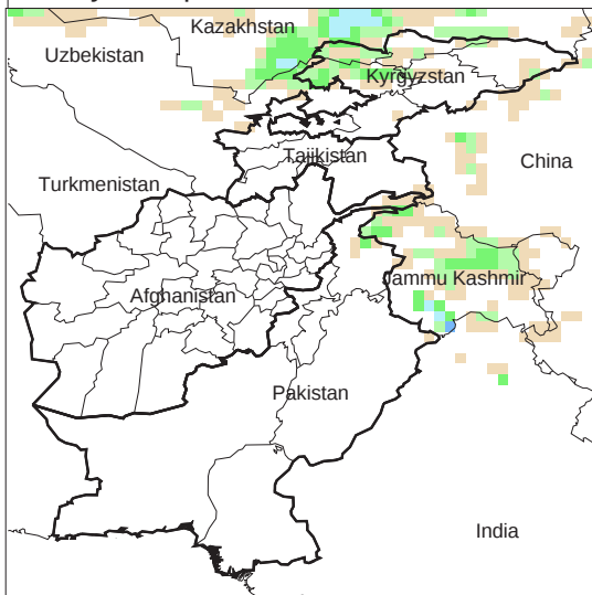
Daily Precip. Forecast for 11 Feb., 2014
