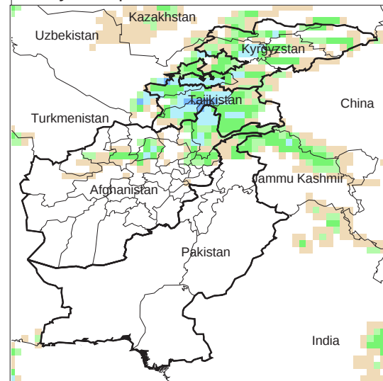
Daily Precip. Forecast for 13 Feb., 2014
