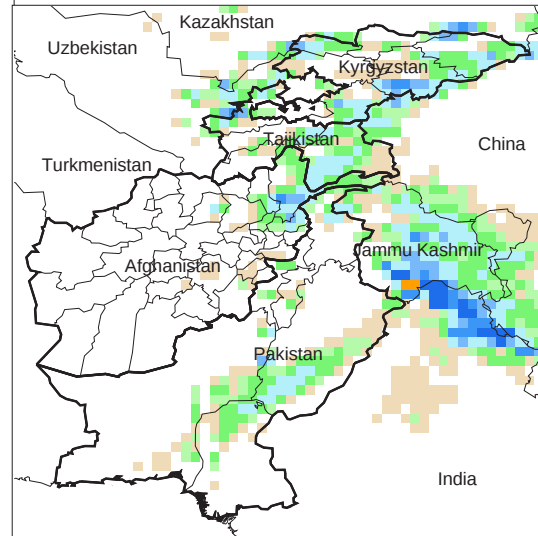
Daily Precip. Forecast for 27 Mar., 2014
