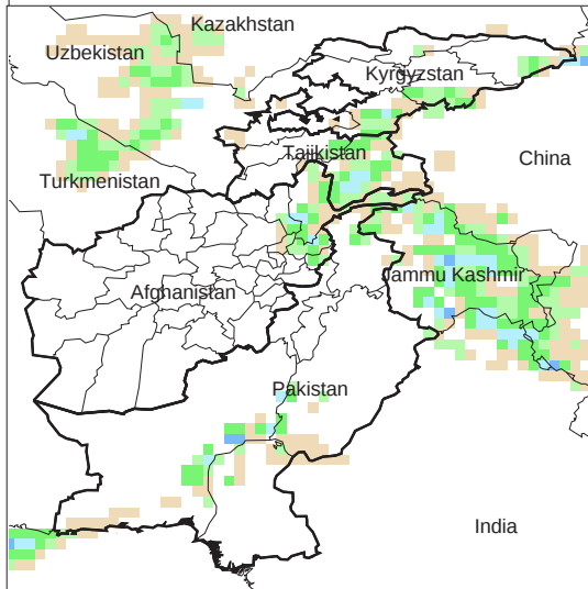
Daily Precip. Forecast for 26 Mar., 2014
