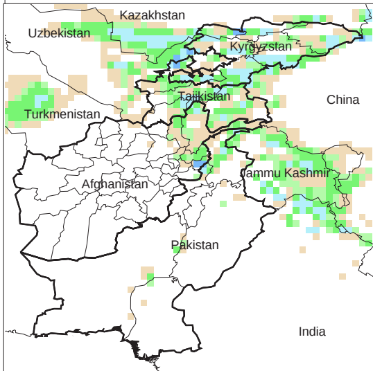
Daily Precip. Forecast for 25 Mar., 2014
