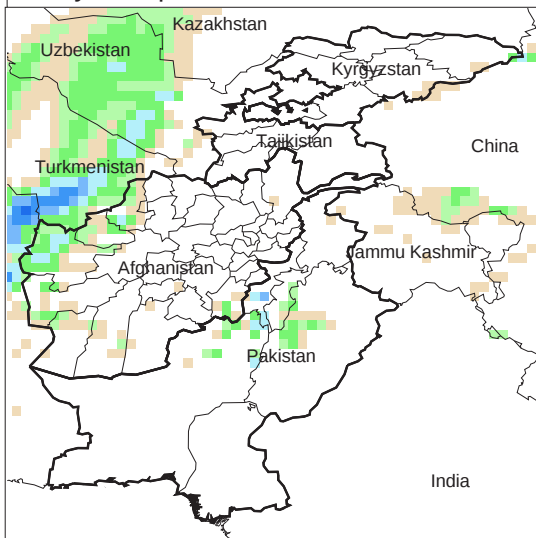
Daily Precip. Forecast for 31 Mar., 2014
