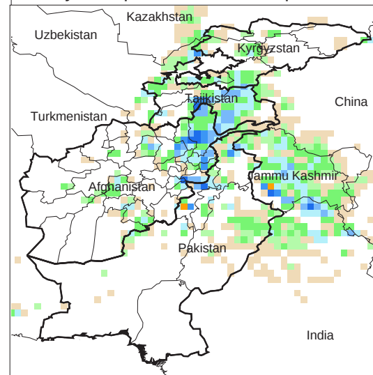
Daily Precip. Forecast for 2 Apr., 2014
