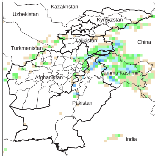
Daily Precip. Forecast for 1 Apr., 2014
