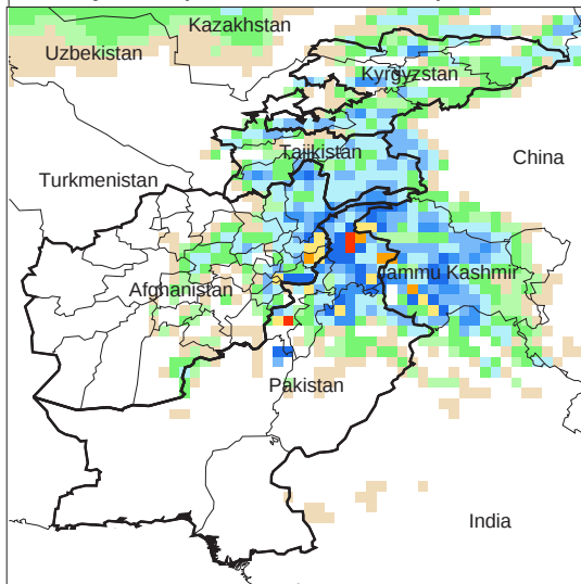
Daily Precip. Forecast for 9 Apr., 2014
