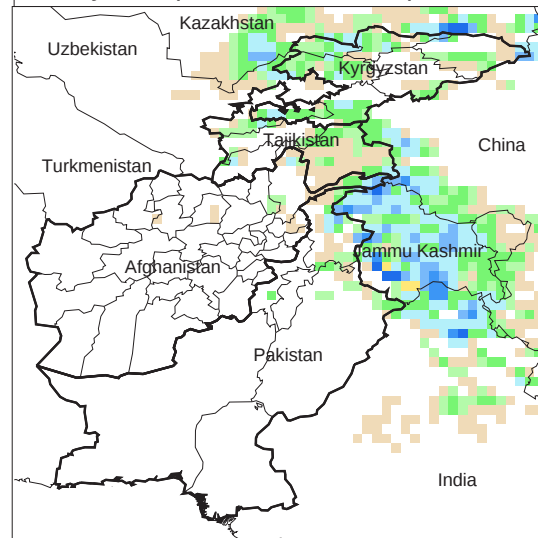
Daily Precip. Forecast for 10 Apr., 2014
