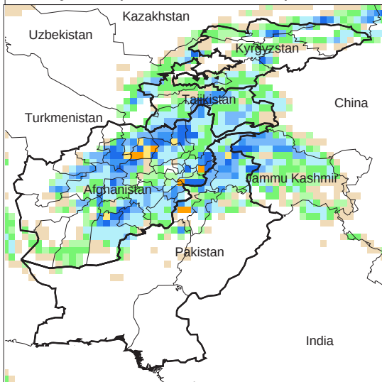
Daily Precip. Forecast for 8 Apr., 2014
