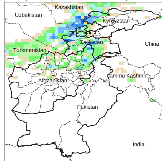
Daily Precip. Forecast for 13 Apr., 2014
