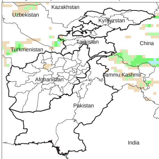
Daily Precip. Forecast for 12 Apr., 2014
