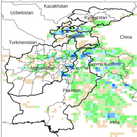
Daily Precip. Forecast for 17 Apr., 2014
