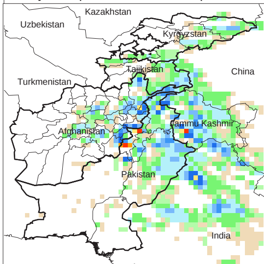
Daily Precip. Forecast for 18 Apr., 2014
