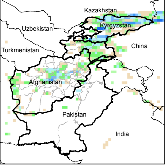
Daily Precip. Forecast for 29 Apr., 2014
