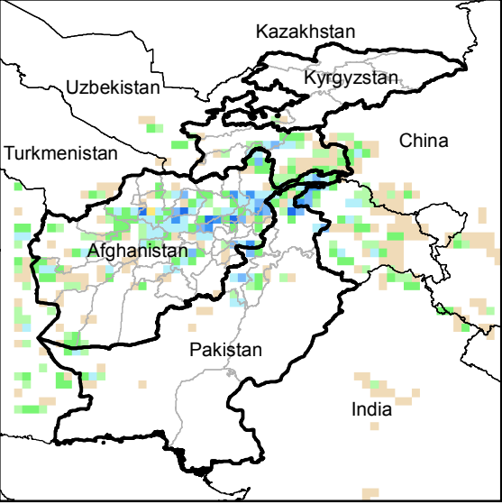
Daily Precip. Forecast for 30 Apr., 2014
