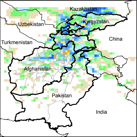
Daily Precip. Forecast for 28 Apr., 2014
