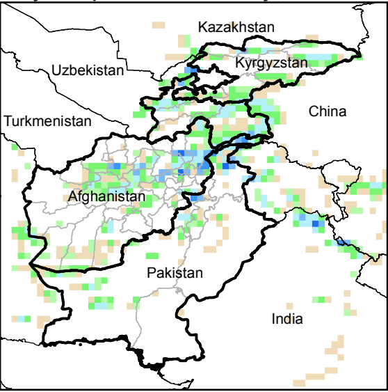
Daily Precip. Forecast for 1 May., 2014
