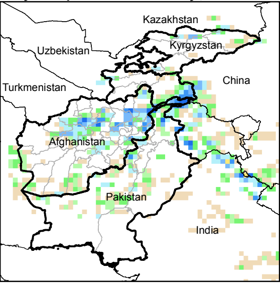
Daily Precip. Forecast for 2 May., 2014
