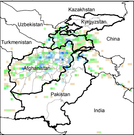
Daily Precip. Forecast for 3 May., 2014
