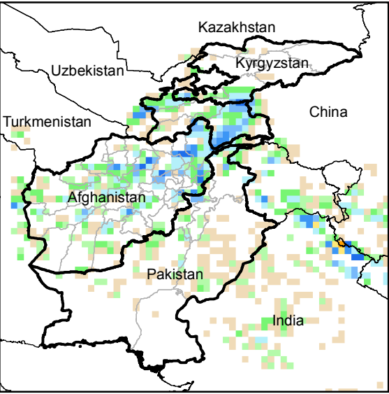
Daily Precip. Forecast for 4 May., 2014
