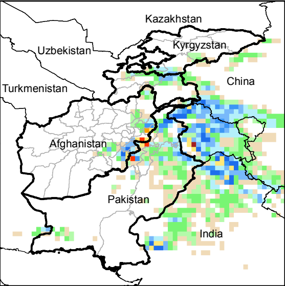
Daily Precip. Forecast for 12 May., 2014
