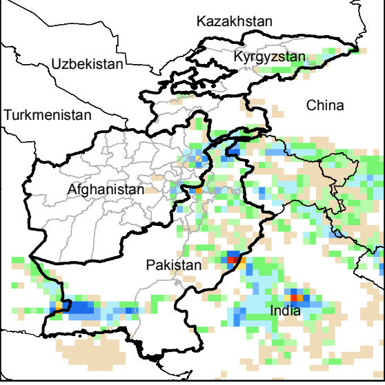
Daily Precip. Forecast for 14 May., 2014
