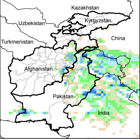
Daily Precip. Forecast for 13 May., 2014
