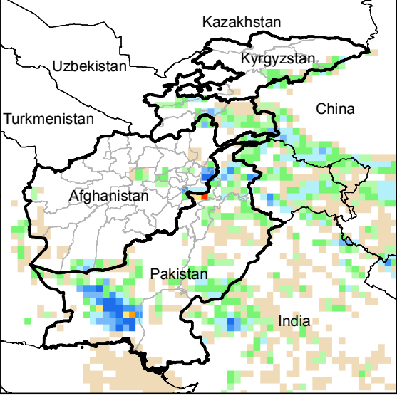
Daily Precip. Forecast for 15 May., 2014
