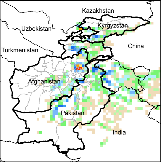
Daily Precip. Forecast for 10 May., 2014
