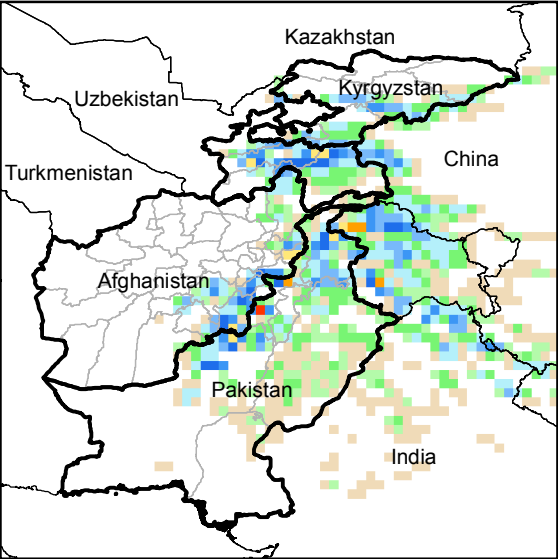
Daily Precip. Forecast for 11 May., 2014
