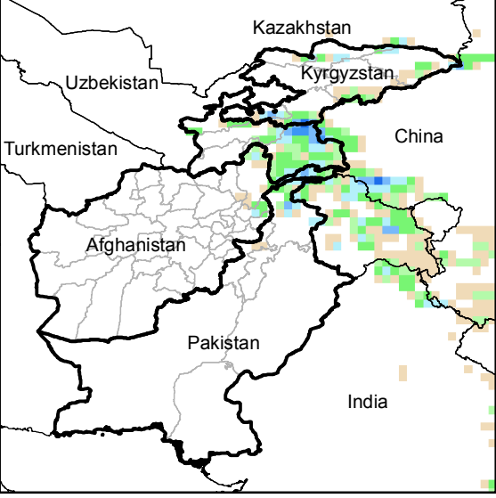
Daily Precip. Forecast for 26 May., 2014
