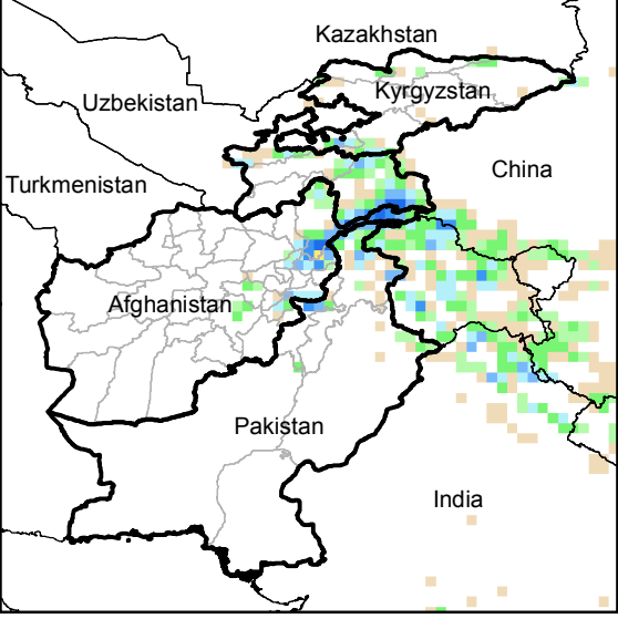
Daily Precip. Forecast for 25 May., 2014
