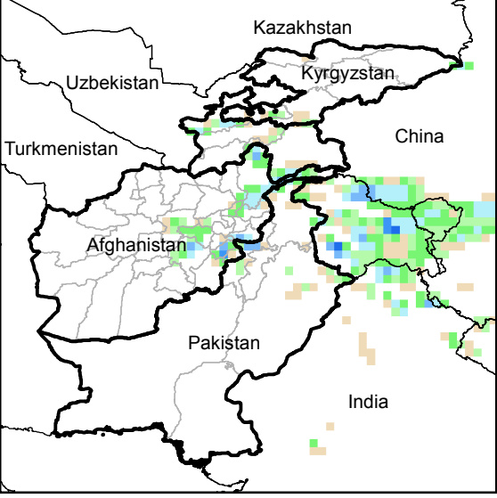
Daily Precip. Forecast for 24 May., 2014
