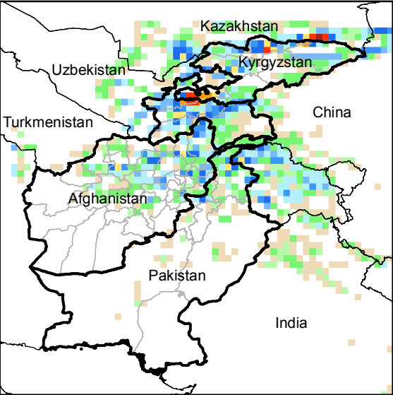
Daily Precip. Forecast for 2 Jun., 2014
