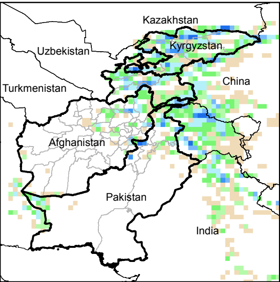
Daily Precip. Forecast for 4 Jun., 2014
