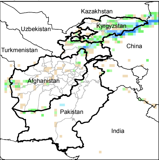
Daily Precip. Forecast for 6 Jun., 2014
