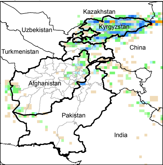
Daily Precip. Forecast for 5 Jun., 2014
