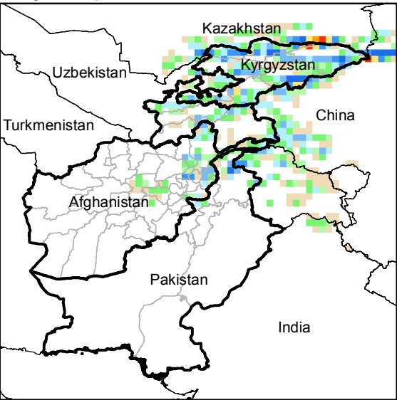
Daily Precip. Forecast for 10 Jun., 2014
