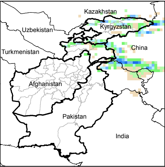
Daily Precip. Forecast for 9 Jun., 2014
