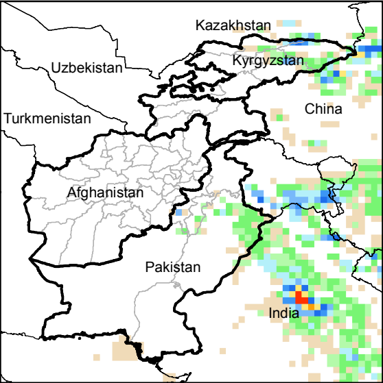
Daily Precip. Forecast for 24 Jun., 2014
