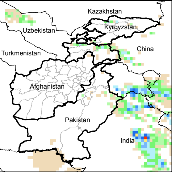
Daily Precip. Forecast for 25 Jun., 2014
