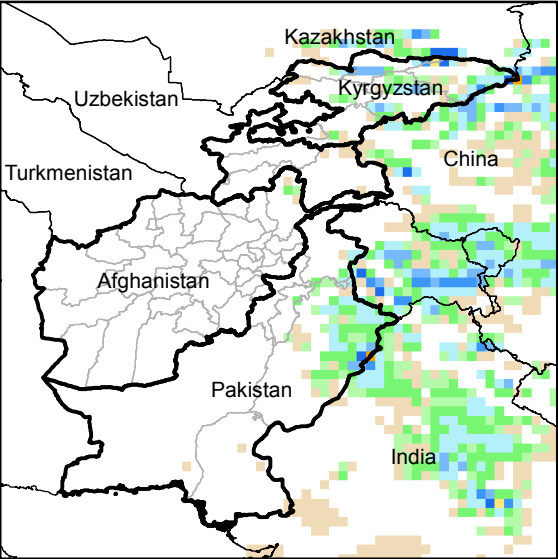
Daily Precip. Forecast for 23 Jun., 2014
