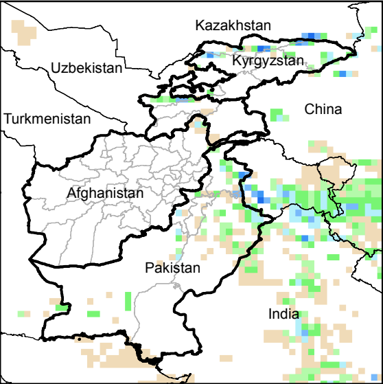
Daily Precip. Forecast for 26 Jun., 2014
