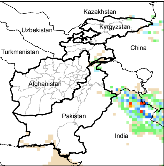
Daily Precip. Forecast for 3 Jul., 2014
