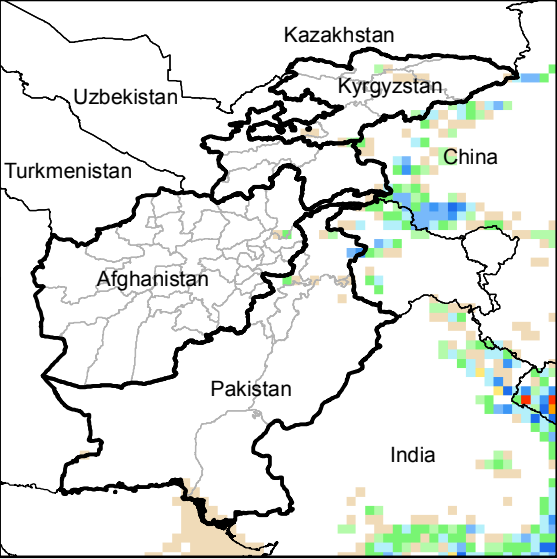
Daily Precip. Forecast for 7 Jul., 2014
