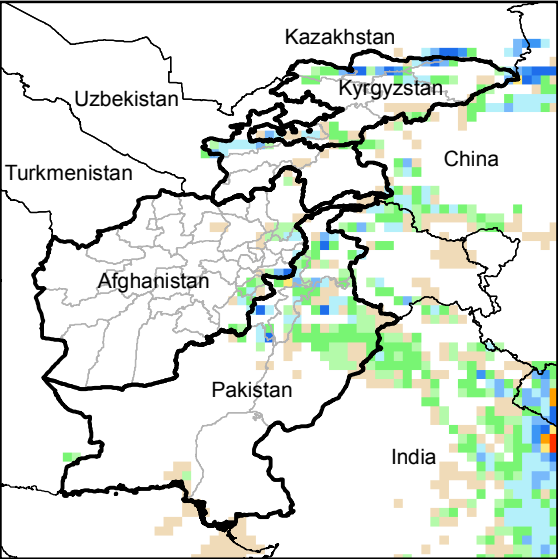
Daily Precip. Forecast for 8 Jul., 2014
