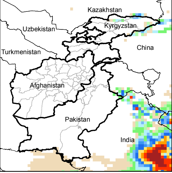
Daily Precip. Forecast for 21 Jul., 2014
