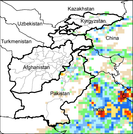
Daily Precip. Forecast for 18 Jul., 2014
