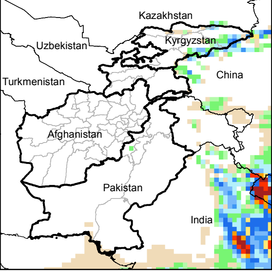
Daily Precip. Forecast for 20 Jul., 2014
