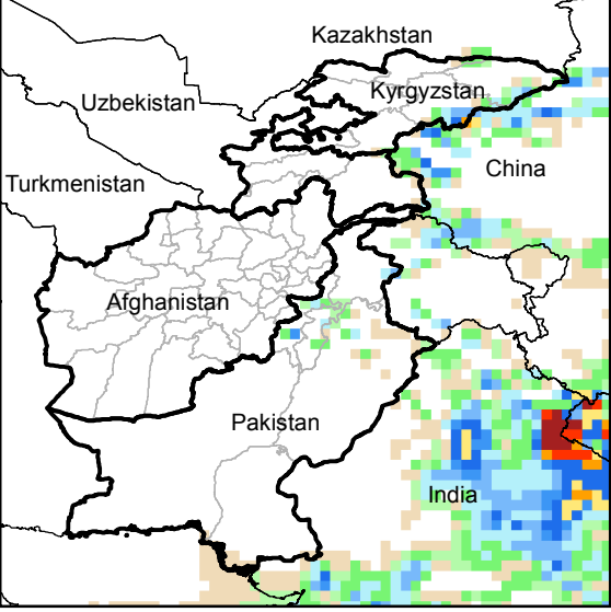
Daily Precip. Forecast for 19 Jul., 2014
