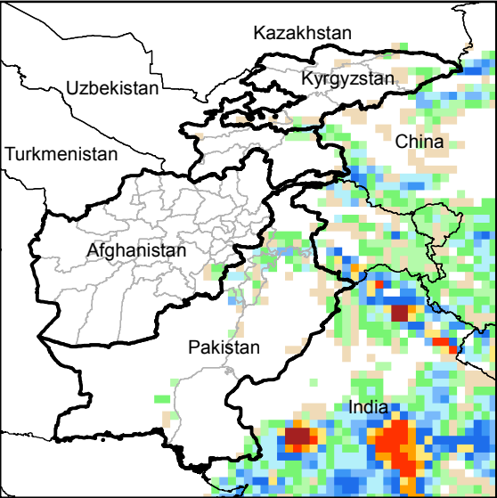
Daily Precip. Forecast for 16 Jul., 2014
