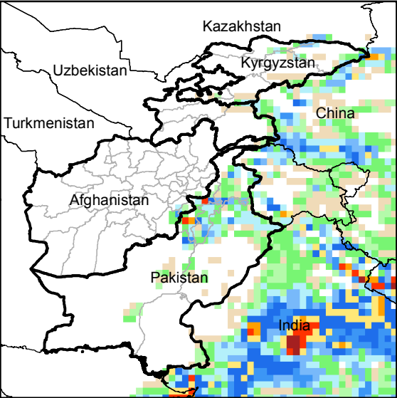
Daily Precip. Forecast for 17 Jul., 2014
