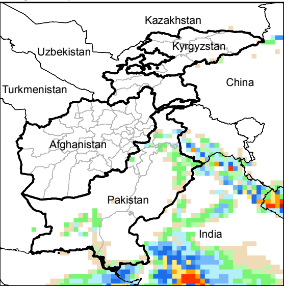
Daily Precip. Forecast for 27 Jul., 2014
