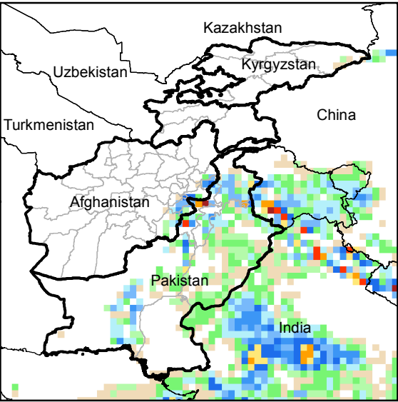
Daily Precip. Forecast for 26 Jul., 2014
