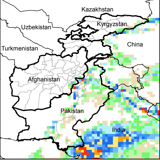
Daily Precip. Forecast for 1 Aug., 2014
