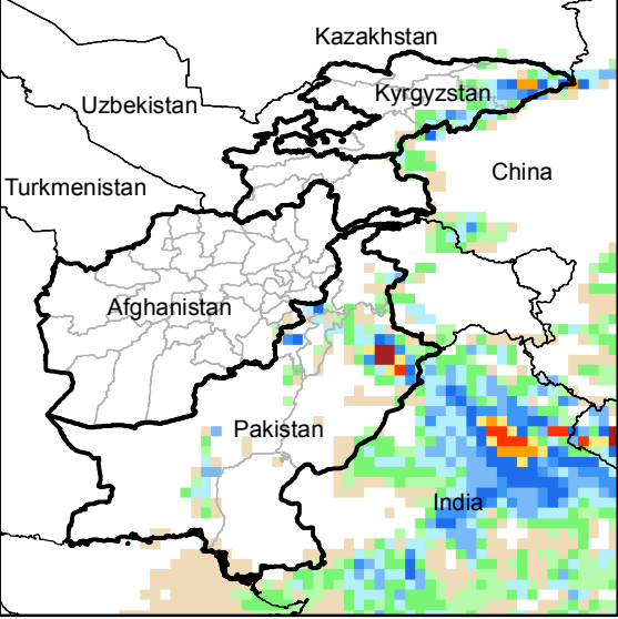
Daily Precip. Forecast for 3 Aug., 2014
