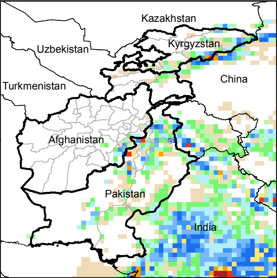
Daily Precip. Forecast for 2 Aug., 2014
