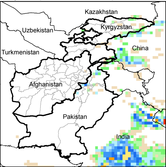
Daily Precip. Forecast for 11 Sep., 2014
