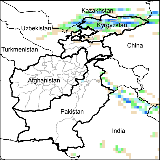
Daily Precip. Forecast for 5 Oct., 2014
