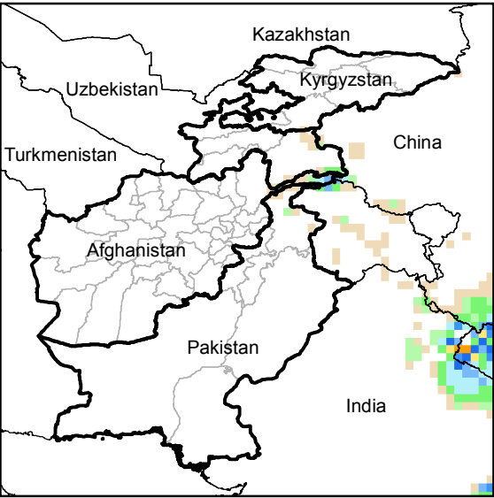
Daily Precip. Forecast for 15 Oct., 2014
