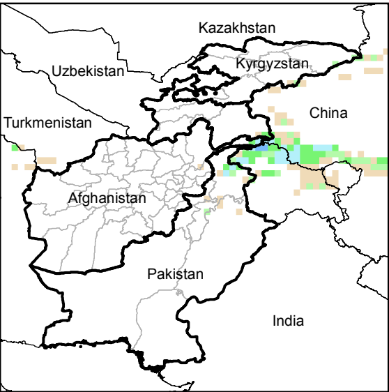
Daily Precip. Forecast for 14 Oct., 2014
