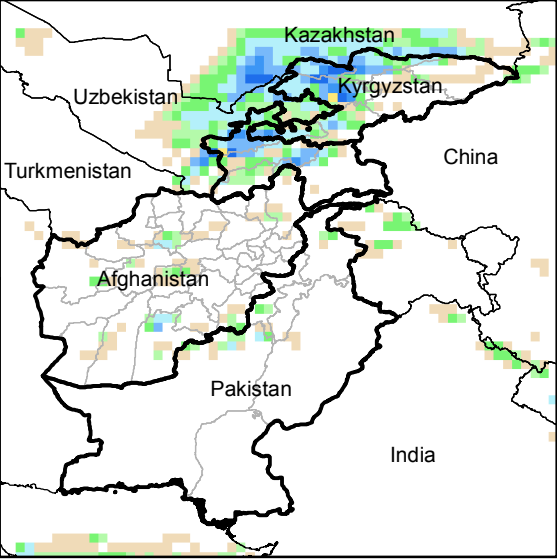
Daily Precip. Forecast for 27 Oct., 2014
