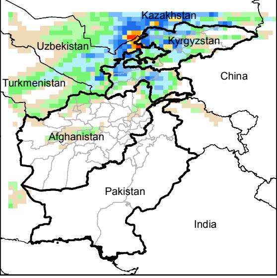
Daily Precip. Forecast for 24 Nov., 2014
