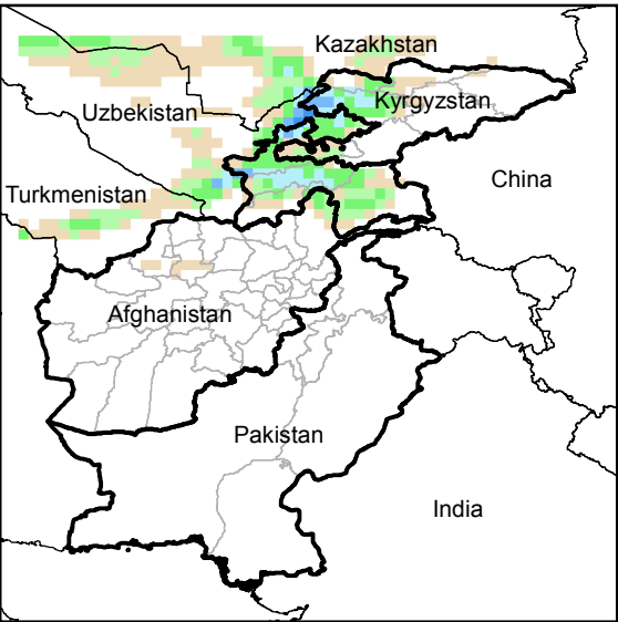
Daily Precip. Forecast for 9 Dec., 2014
